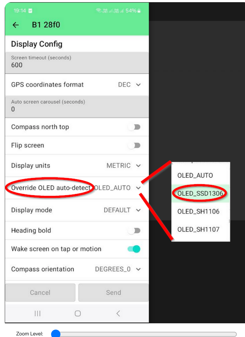
Figure 16: Change display settings
