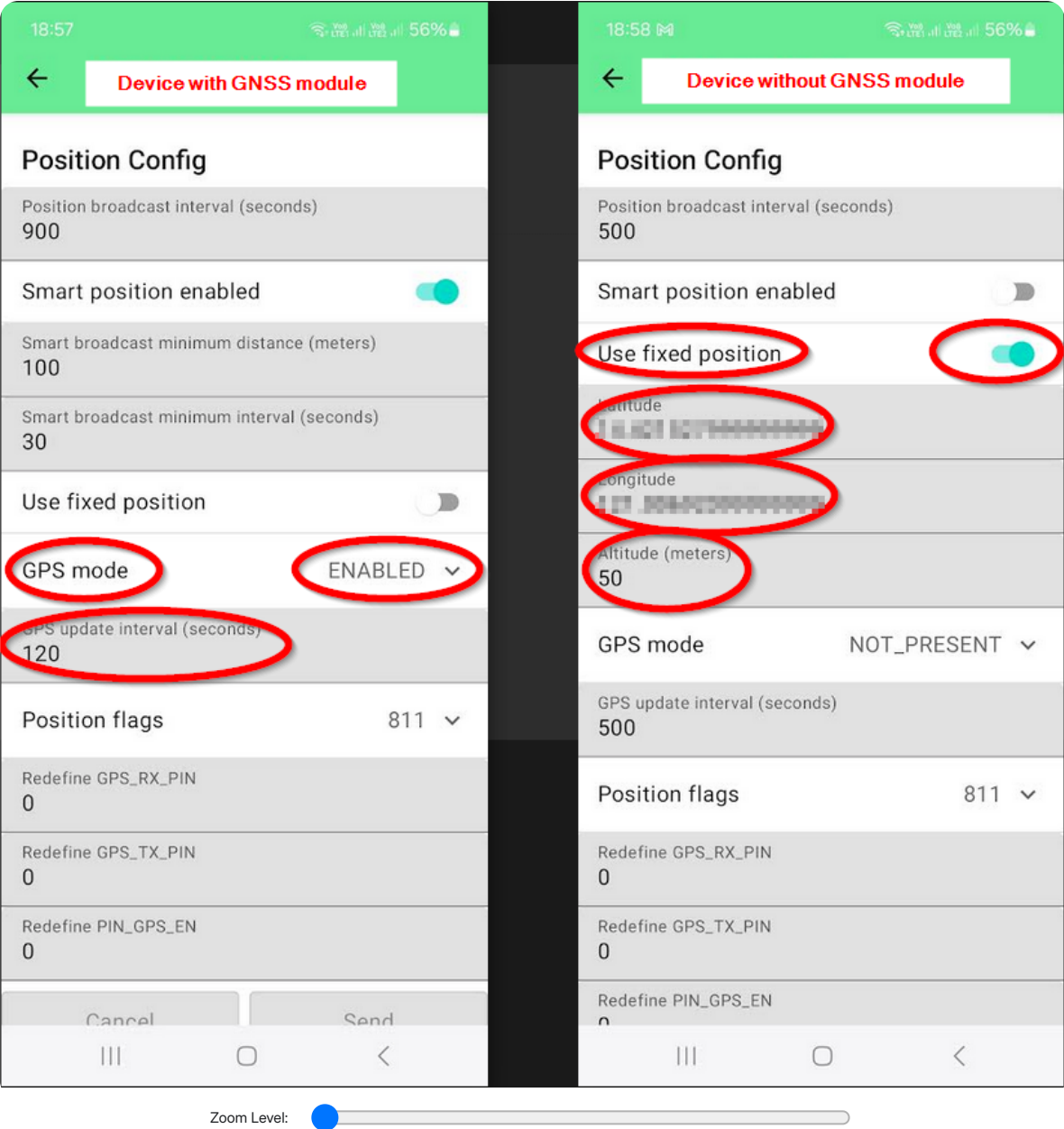
Figure 14: Location settings
