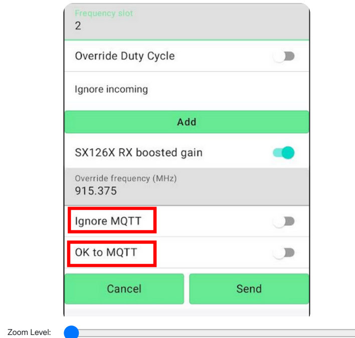
Figure 13: MQTT settings
